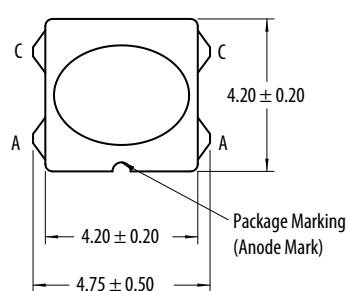
Package Drawing D
